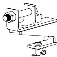
Pivot Bracket for 60" Coupler
