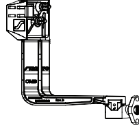
Coupler Mounted Bracket, 45° Trainline Support Casting with Flange
